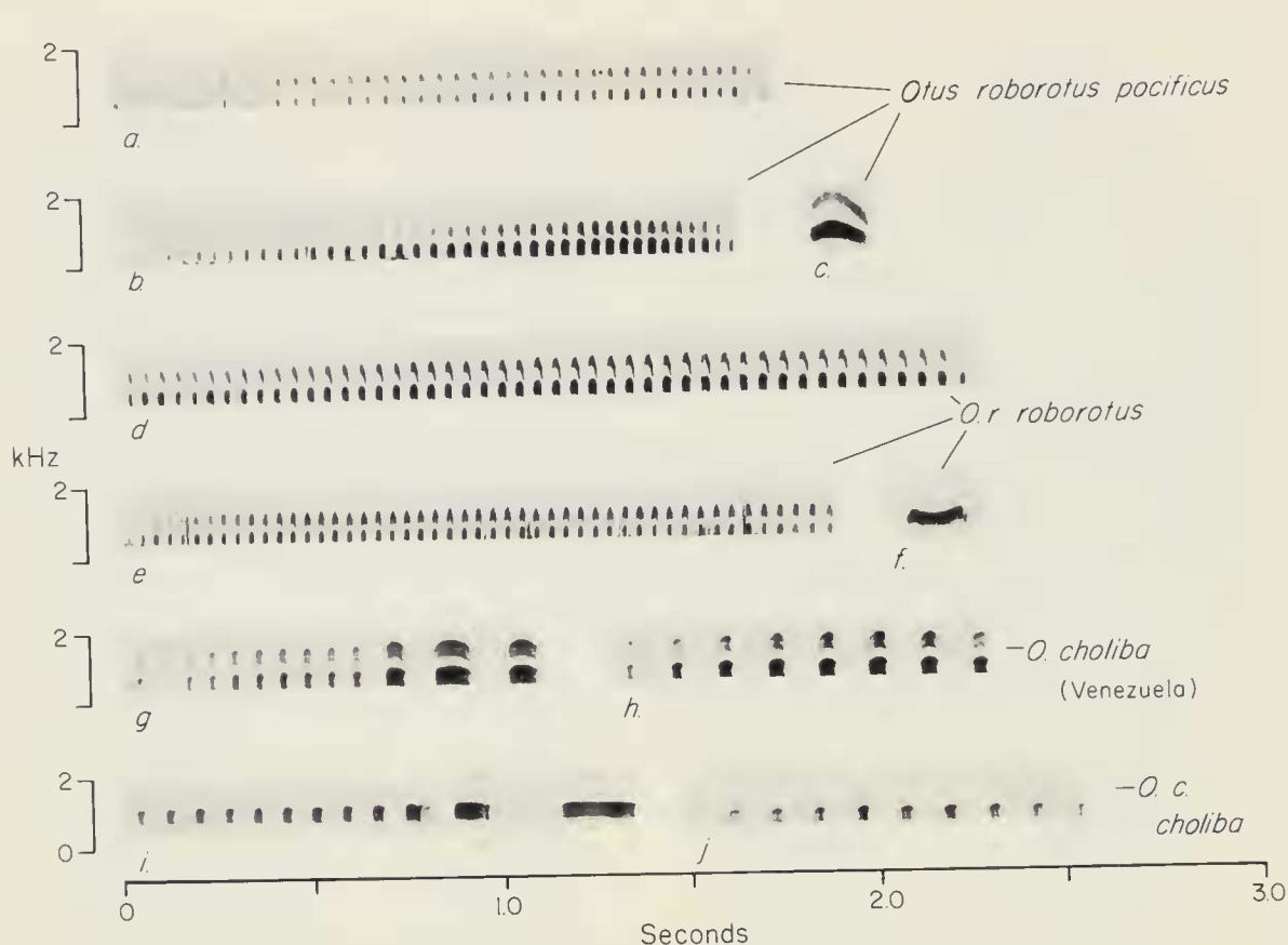
FIG. 3. Audiospectrograms of tape recordings of the common vocalizations of Otus roborotus and Otus choliba . (a) Advertising song of O. r. pacificus (MVZ tape 16, cut 7, cue 11), recorded by the authors at Parinas, 100 feet elevation, 7 km N and 15 km E. Talara, Depto. Piura, Perú, on October 29, 1974. (b) Advertising song of O. r. pacificus (MVZ tape 16, cut 8, cue 1), recorded by the authors at Quebrada Bocapan, 50 feet elevation, 6 km S and 4 km W of Zorritos, Depto. Tumbes, Perú, on October 30, 1974. (c) Bark of same male as recorded in b (cue 23). (d) Advertising song of O. r. roborotus (MVZ tape 15, cut 3, cue 2) recorded by the authors at 5 miles SSE Jaen, 3000 feet elevation, Depto. Cajamarca, Perú, on August 22, 1970. (e) Advertising song of O. r. roborotus (MVZ tape 15, cut 6, cue 26) recorded by the authors at 10 km WSW Bagua Chica, 1700 feet elevation, Depto. Amazonas, Perú, on August 31, 1970. (f) Bark of same individual recorded in e (cue 14). (g) Advertising song with terminal barks of Otus choliba , recorded by Paul Schwartz in Venezuela. Subspecies, exact locality, and date unknown. (h) Advertising song lacking terminal barks in Otus choliba . Same individual as in g. (i) Advertising song of Otus choliba choliba (MVZ tape 94, cut 2, cue 1), with terminal barks. Recorded by Victoria Dziadosz at El Tirol, 230 meters elevation, 19.5 km by road NNE Encarnacion, Depto. Itapua, Paraguay, on September 15, 1978. (j) Advertising song of Otus choliba choliba (MVZ tape 94, cut 1) in which the terminal emphatic notes (barks) are lacking. Same recordist, locality, and date as in i.
